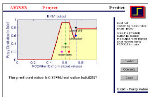
Fig.3. The output of the Explicit Knowledge Module for the given input data set.
