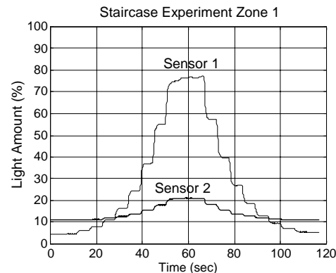
Fig. 3. Staircase Experiment in Zone #1
