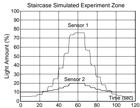
Figure 15: Simulated Staircase Experiment Zone #1
