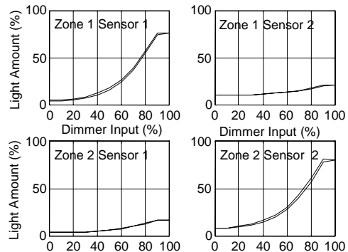
Figure 8: Static Characteristics
