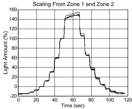
Fig. 5. Scaled Staircase Result (Zone #1 and #2)
