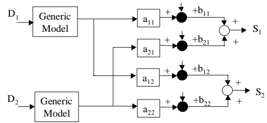
Fig. 7. Simplified 2X2 Structure
