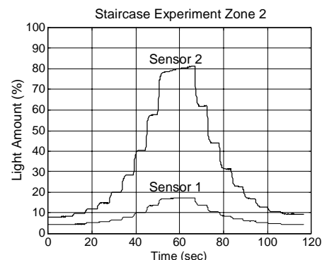
Fig. 4. Staircase Experiment in Zone #2
