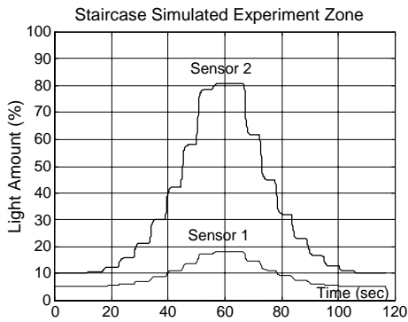
Fig. 16. Simulated Staircase Experiment Zone #2
