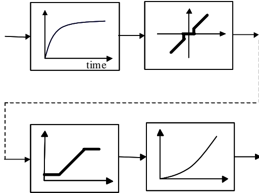
Fig. 10. Components of Generic Static Model
