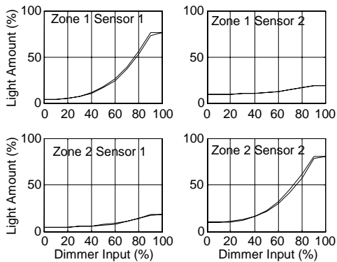
Fig. 17. Simulated Static Characteristics
