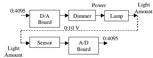
Fig. 2. I/O Block Scheme
