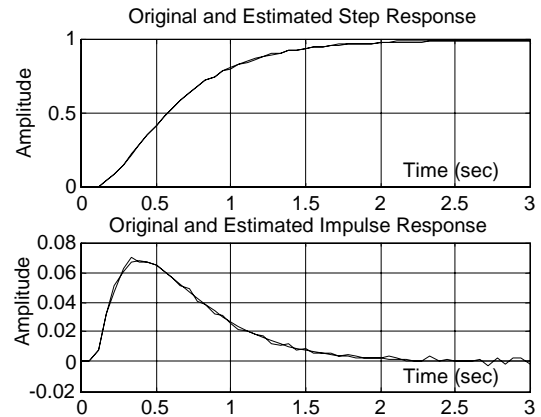
Fig. 12. Real & Estimated Step and Impulse Responses used in the Dynamic Model
