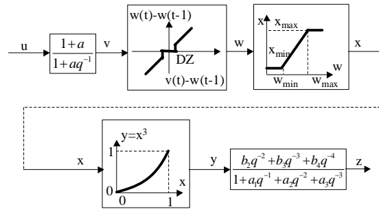
Fig. 14. Internal Structure of the Generic Model
