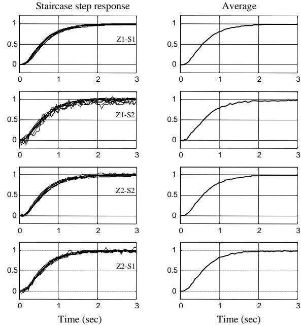
Fig. 11a,b. Dynamic & Averaged Characteristics
