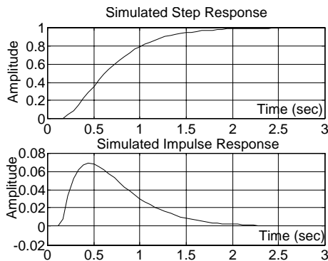
Fig. 18. Simulated Dynamic Characteristics
