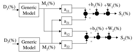
Fig. 13. Simulator Structure
