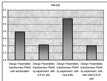
Fig. 6. Global influences of variation of parameters + a combination of transformers from different generations + supply voltage variation on TAC; a combination of transformers from different generations + supply voltage variation on TAC; supply voltage in case of using the combination of transformers from different generations on TAC
