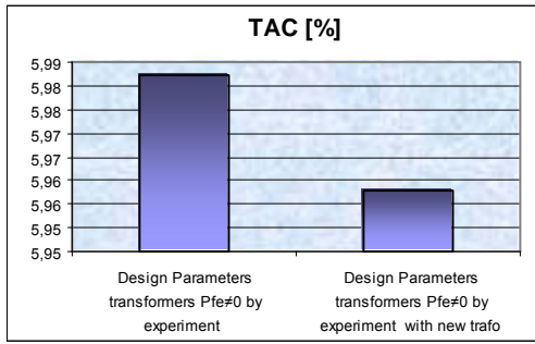
Fig. 5. Influence of using different generations transformers on TAC
