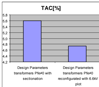
Fig. 3. Influence of supply voltage on TAC
