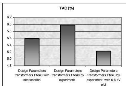
Fig. 4. Global influence (parameters + supply voltage) and supply voltage influence - in the situation of real transformers – on TAC
