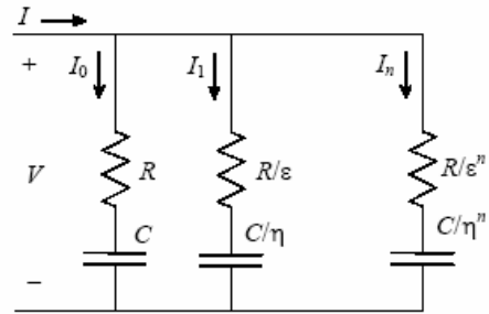
Fig. 8. Recursive circuit scheme.
