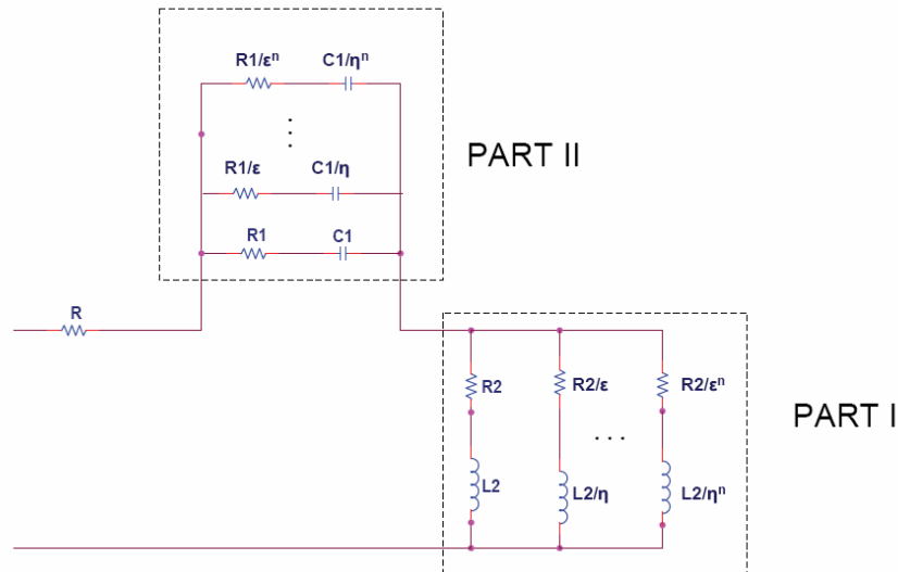
Fig. 10. The corresponding implementation of the fractional-order model is an equivalent higher order circuit.
