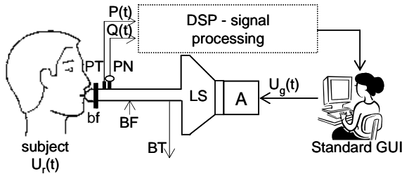
Fig. 1. Standard FOT set-up.
