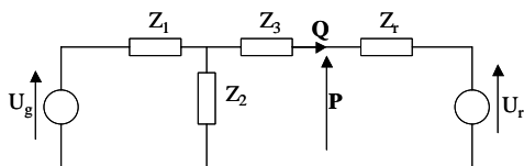
Fig. 3. Electrical scheme analogy.
