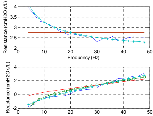
Fig. 7. Asthmatic subject case. (---): non-parametric model from (4); (o): the integer-order RLC model (5); (-): integer-order RLC-A model (6); (*) the fractional-order RLC\alpha\beta model (7).
