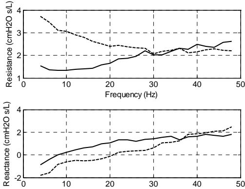
Fig. 4. Respiratory impedance: healthy (continuous line) and asthmatic (dashed line) subject.
