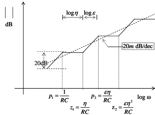
Fig. 9. Pole-zero location for the admittance.
