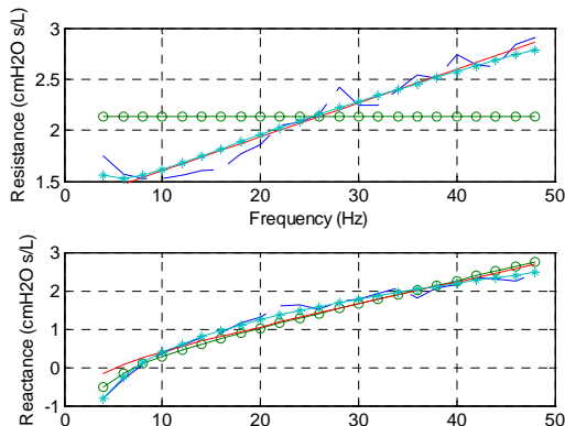
Fig. 6. Healthy subject case. (---): non-parametric model from (4); (o): the integer-order RLC model (5); (-): integer-order RLC-A model (6); (*) the fractional-order RLC\alpha\beta model (7).
