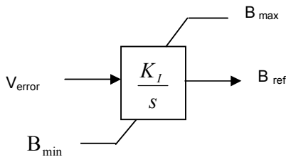
Fig.4. Measuring model.
