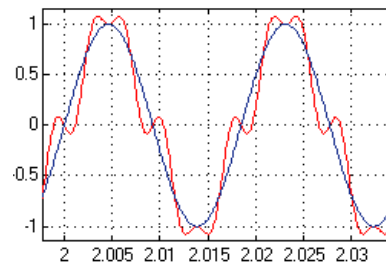
Fig.10. Detail of the synchronised input and output
