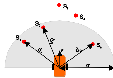
Fig.3. Notations used to describe virtual pheromones aggregation and diffusion
