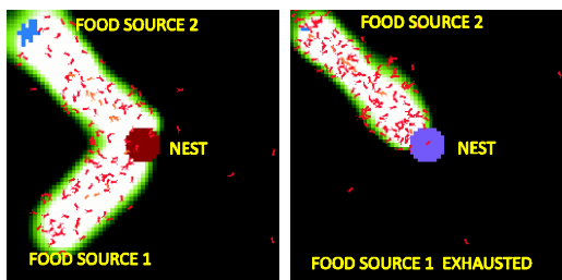
Fig.1. A simulation of ant colony activity using Netlogo. Lighter shades of green indicate higher pheromone concentrations
