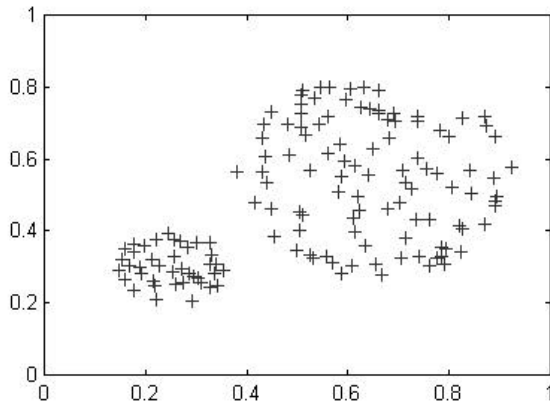
Fig. 3. Data set I, with two spherical clusters
