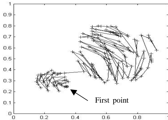
Fig. 4. The ordered data set, starting from x_1
