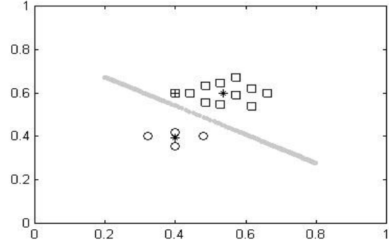
Fig. 16. Clustering of the data set IV, with PFBA
