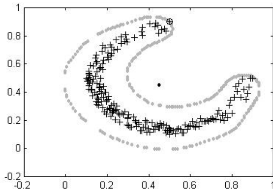
Fig. 9. Constant potential surface for \alpha = 80
