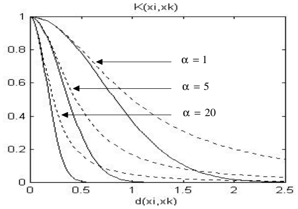
Fig. 1. Potential functions for three values of \alpha
