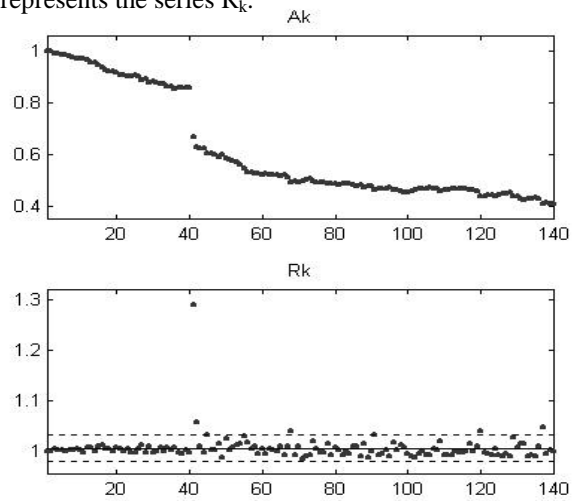
Fig. 6. The series A_k and R_k with the start point x_1
