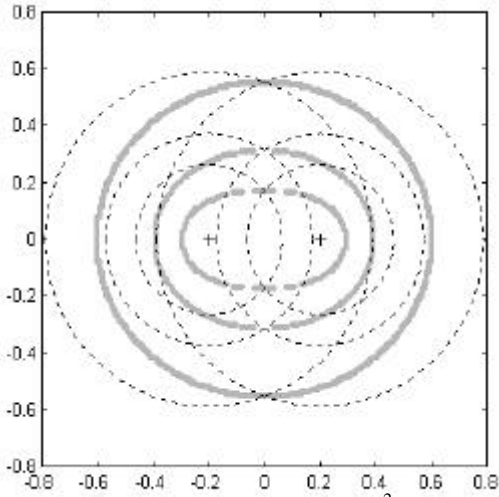
Fig. 2. Constant potential surfaces in \mathbb{R}^2 space
