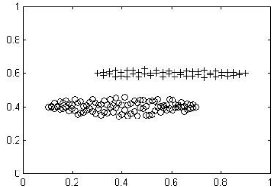
Fig. 10. Clustering elongated shapes with PFBA
