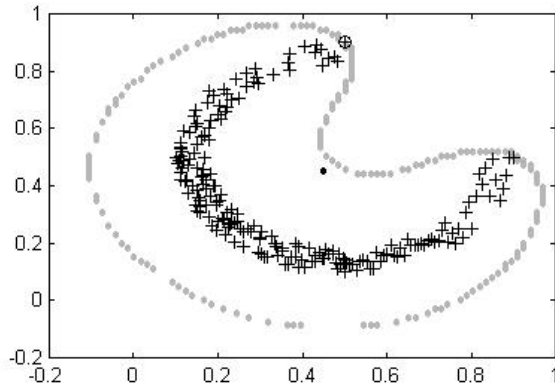
Fig. 8. Constant potential surface for \alpha = 25
