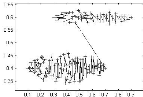
Fig. 11. The ordered data set II, starting from x_{60}
