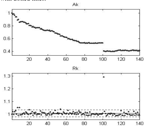
Fig. 7. The series A_k and R_k with the start point x_{120}
