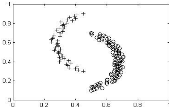
Fig. 13. Clustering irregular shapes with PFBA
