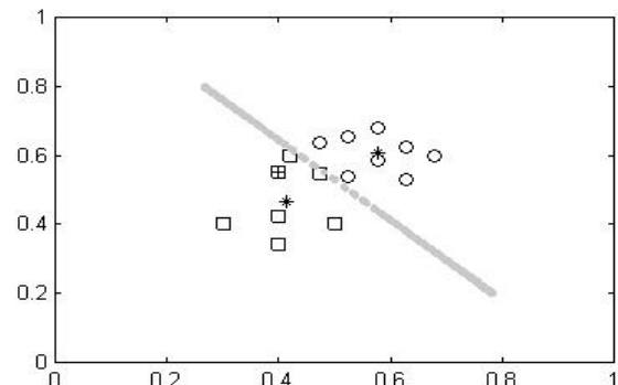
Fig. 17. Noisy set clustering with ISODATA
