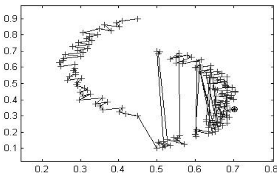
Fig. 15. The ordered data set III, starting from x_{60}
