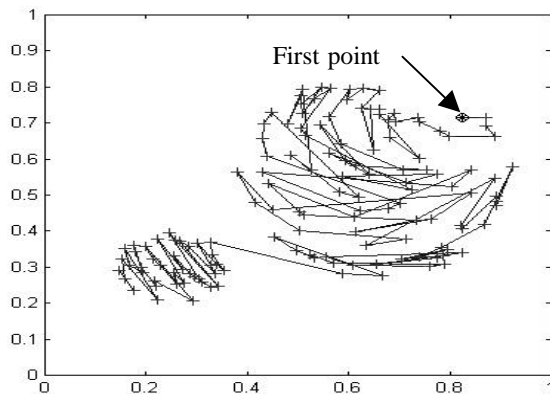
Fig. 5. The ordered data set, starting from x_{120}
