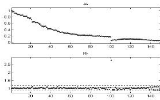
Fig. 12. The series A_k and R_k for ordered data set II
