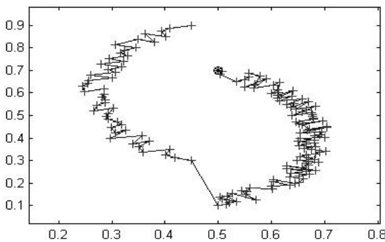
Fig. 14. The ordered data set III, starting from x_1
