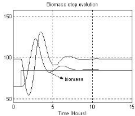
Fig. 6. Time evolution to the operational point
