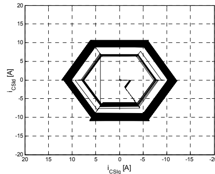
Fig. 7. CSI-current space-phasor diagram in the stator-fixed reference frame.
